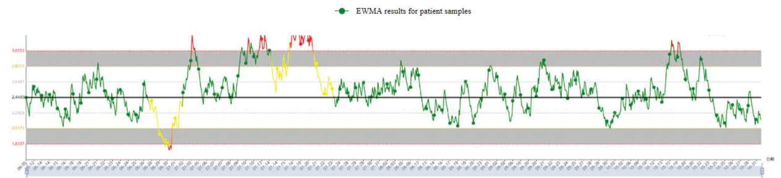
DXI800 AMH 0.02-10.14 EWMA chart (Tradition-PBRTQC \lambda: 0.03 )
