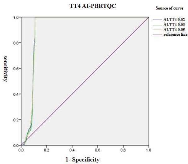
Attached Figure 2 The ROC curve of the EWMA algorithm describes the different weighting factors in Supplementary
